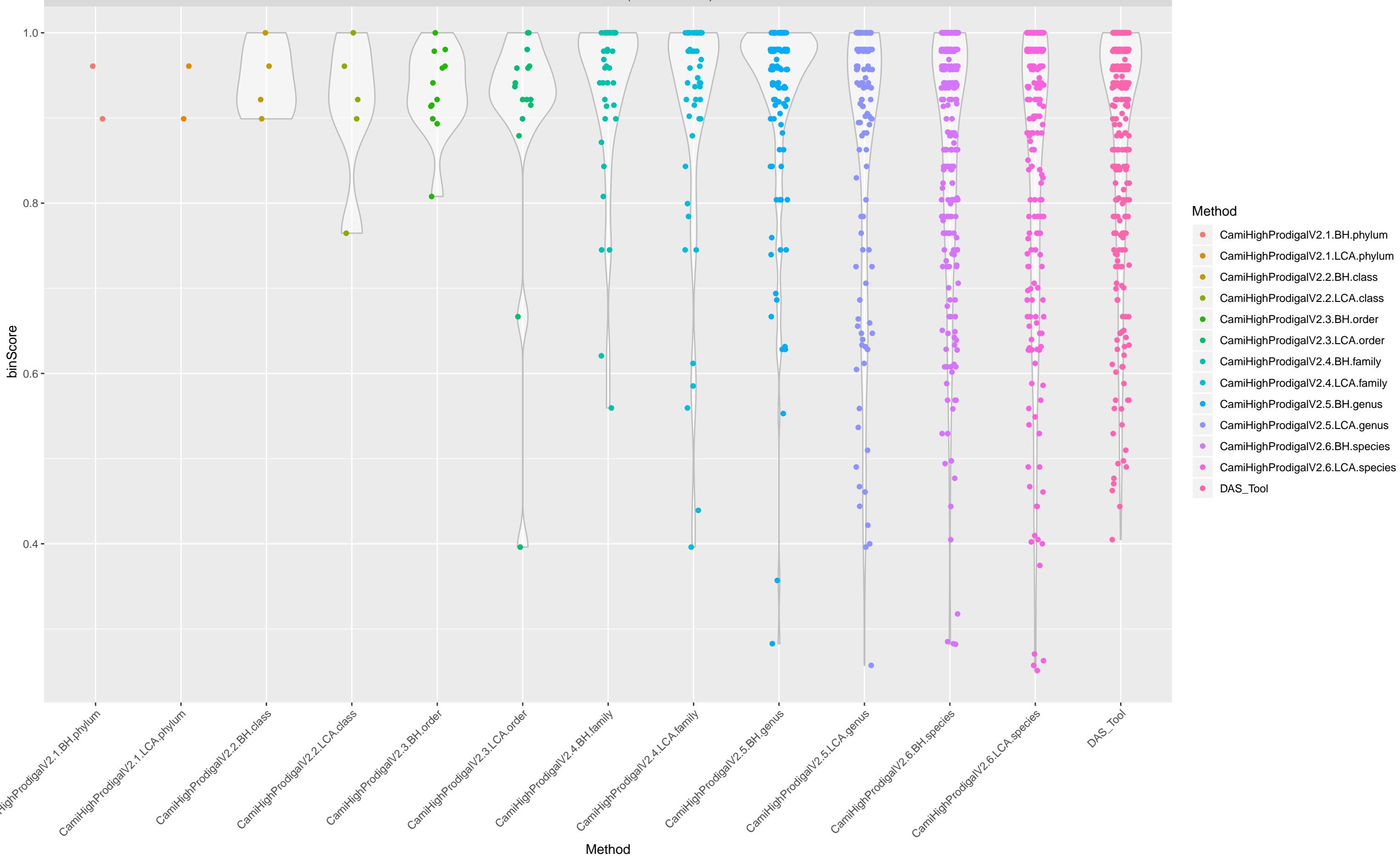
Score distribution of bins (BinScore &gt; 0.25)
